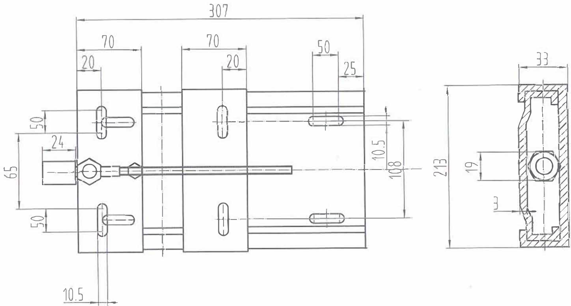
SMA 307 Slide Base Dimensional Data
